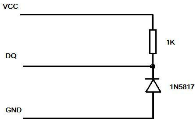
1-wire 尾端匹配电路
